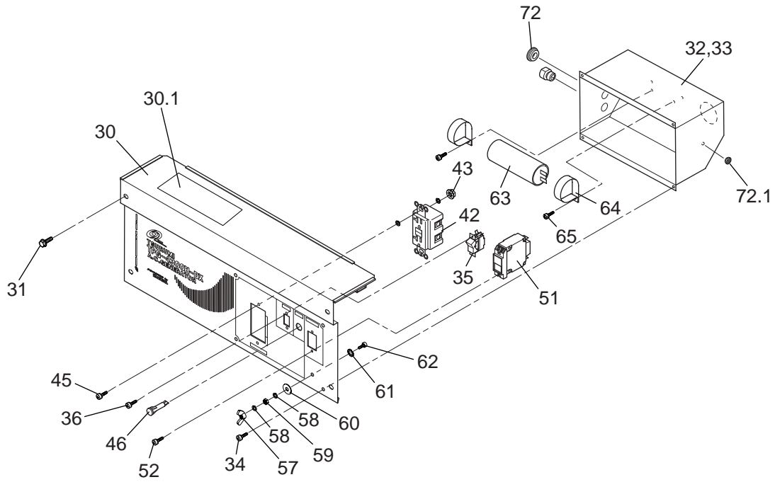
FRONT PANEL
