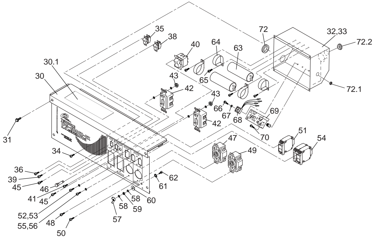
FRONT PANEL
