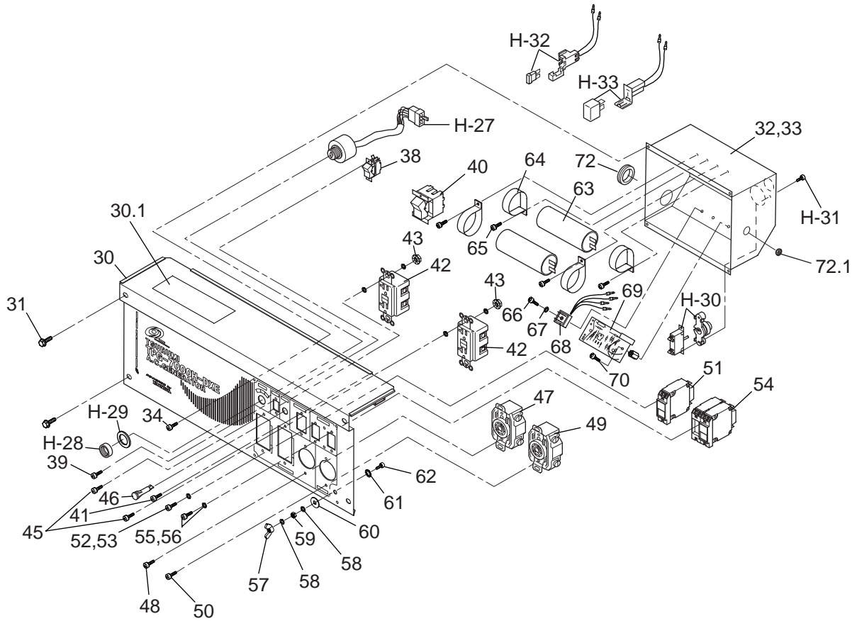
FRONT PANEL
